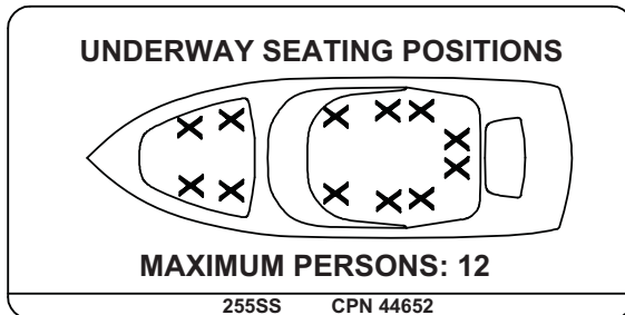
Figure 7-4: Seating Positions
