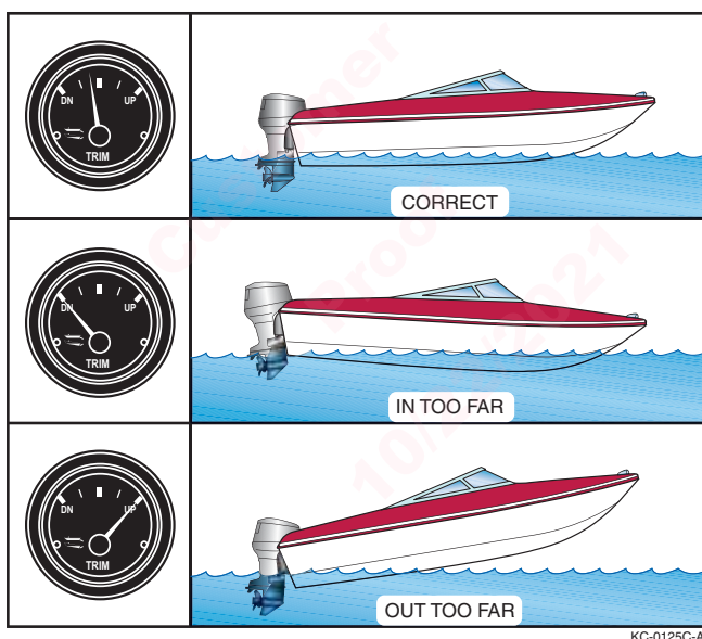
Figure 7-12: Power Trim
