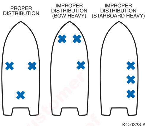
Figure 7-1: Weight Distribution
