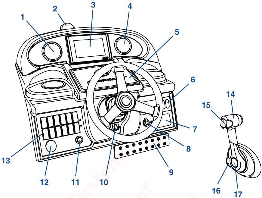
Figure 10-6: 264CR
