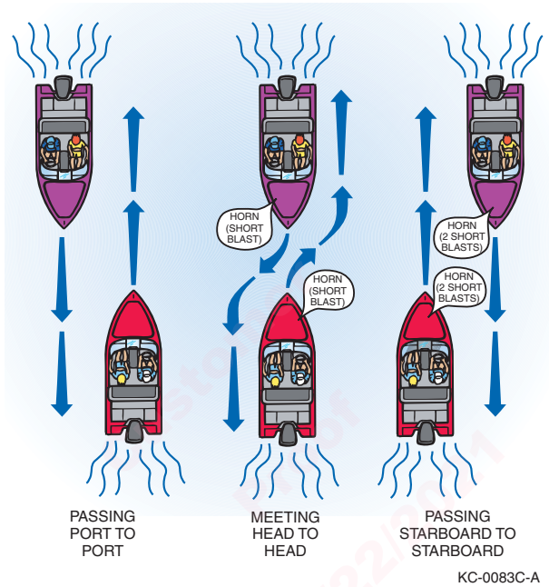
Figure 6-2: Meeting Head-On
