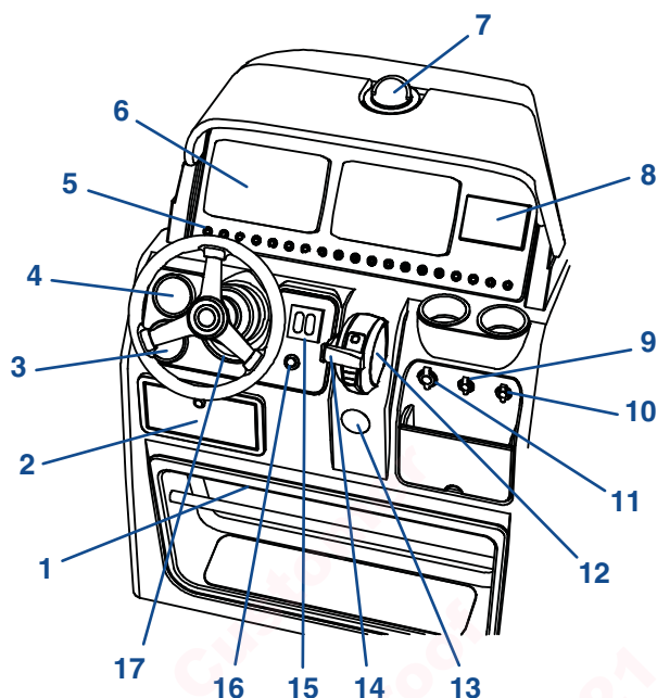
Figure 10-1: FINSEEKER 200CC/210CC/220CC/230CC
