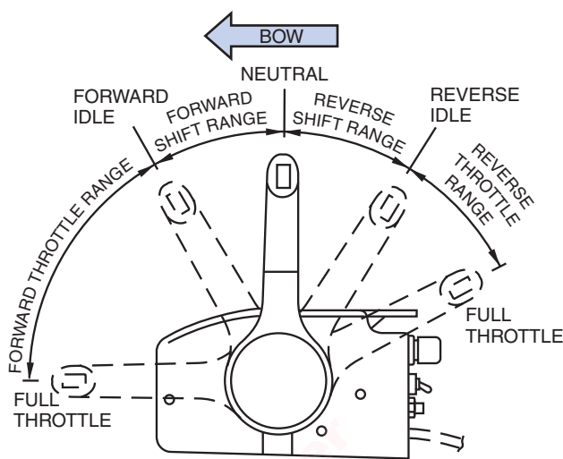
Figure 10-8: Single-Lever Controls
