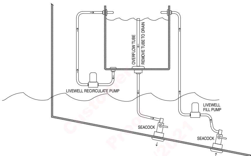
Figure 9-12: CROWLINE/FINSEEKER Livewell/Baitwell
