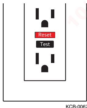
Figure 9-9: Testing GFCI Receptacles
