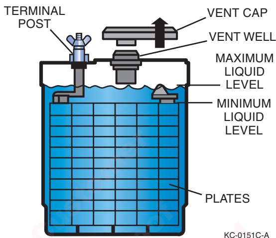
Figure 11-3: Lead-Acid (Wet Cell) Battery
