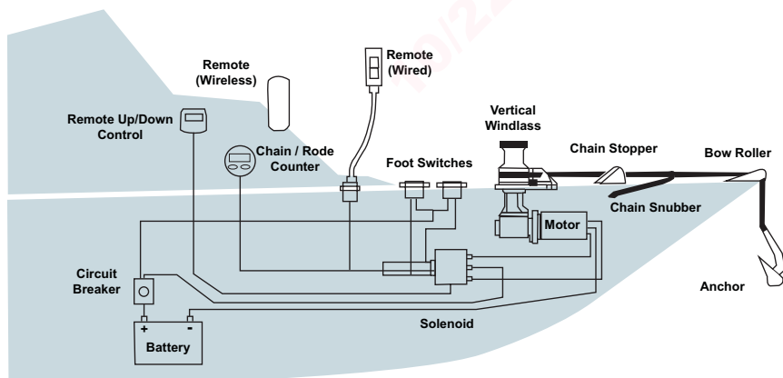
Figure 9-10: Windlass
