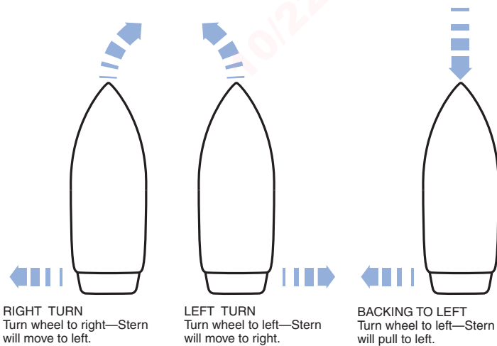
Figure 7-10: Steering Patterns
