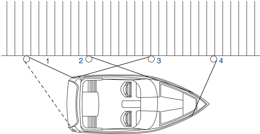
Figure 7-17: Mooring Lines
