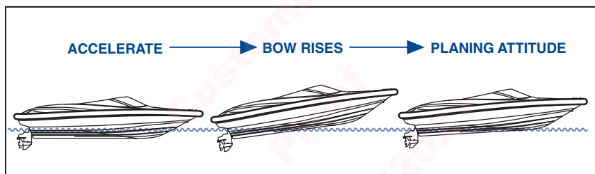
Figure 7-11: Boat Attitude
