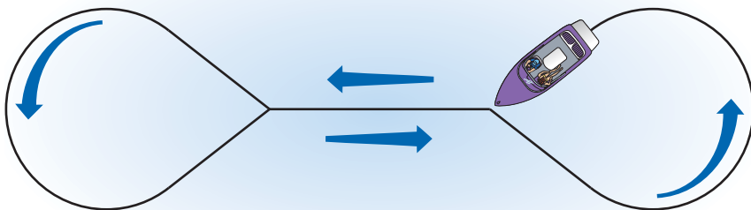
Figure 2-13: Dog-Bone Pattern
