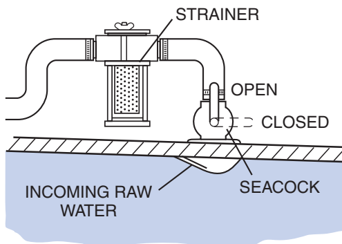
Figure 9-13: Typical Seacock and Strainer
