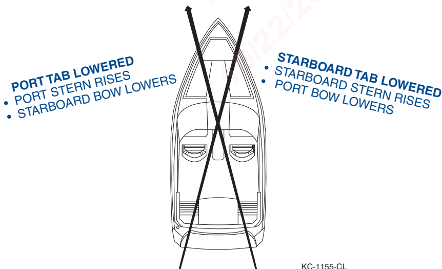
Figure 7-13: Trim Tabs
