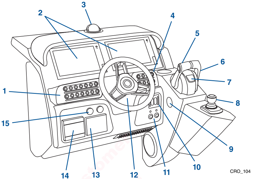
Figure 10-2: FINSEEKER/CROWLINE 260DC/280DC
