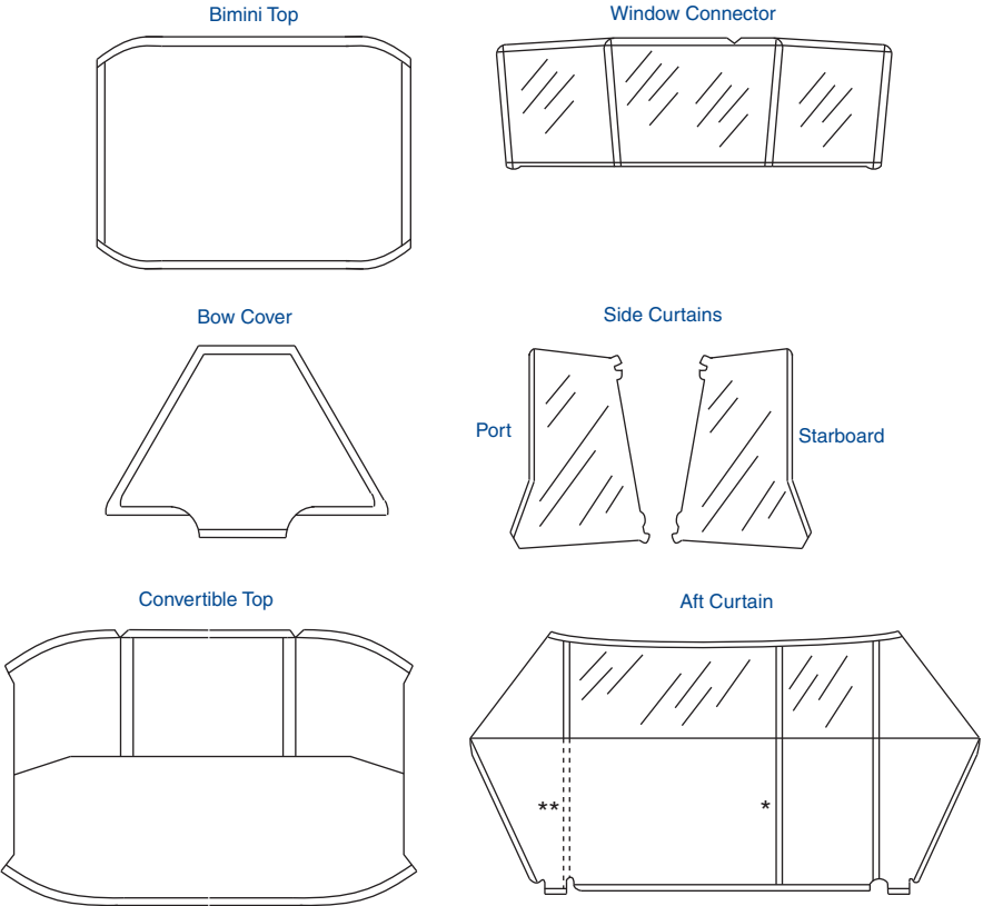
Figure 3-28 Camper Top Shown
