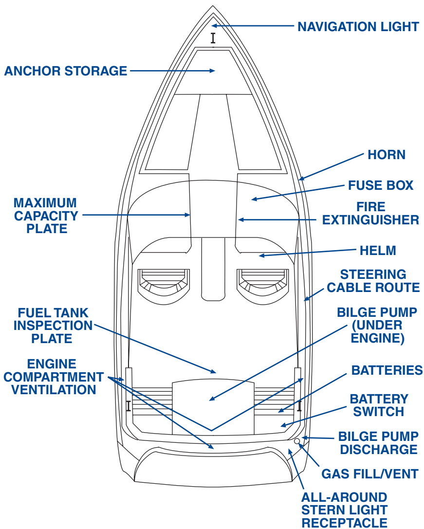
Figure 6-1 Typical Stern Drive Equipment
