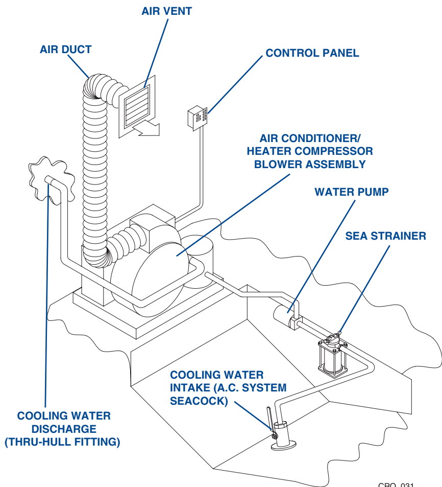
Figure 4-6 Typical Air Conditioning System
