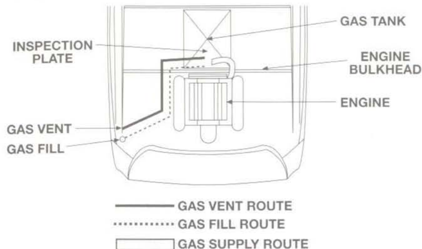
FIGURE 4.3 TYPICAL STERNDRIVE GAS SYSTEM (NOTE: SOME MODELS WILL HAVE A FILL/VENT COMBINATION)
